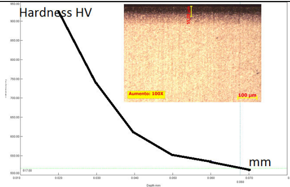
Plasma Nitriding for aluminium injection dies
